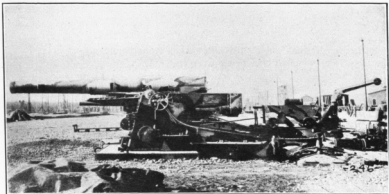
FIG. 9.—United States 240-mm. howitzer, model 1918
