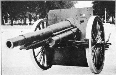
FIG. 12.—United States 4.7-inch gun and carriage, model 1906. This gun throws a projectile weighing 45 pounds a distance of about 6 miles
