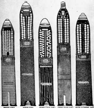
FIG. 15.—Types of shrapnel in modern use
