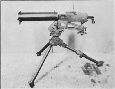
FIG. 56.—Browning heavy machine gun, model 1917
