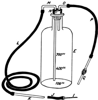
FIG. 107.—Transfusion apparatus. J , Rubber tube; K , glass tube; L , rubber tube; M , glass tube; N , rubber stopper; O , glass tube; P , rubber tube; Q , glass tube for exerting compression (cotton in bulb)
