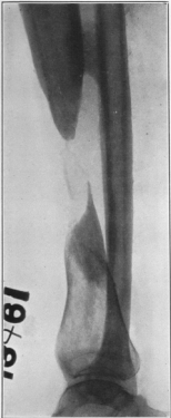
FIG. 115.—Case 11. Roentgenogram showing loss of substance
