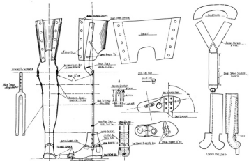
FIG. 145.—Mechanical drawing of the provisional apparatus for below-the-knee amputation used in the American Expeditionary Force.
