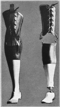
FIG. 172.—Letterman General Hospital artificial leg, assembled and unassembled
