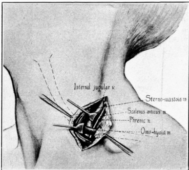
FIG. 190.—Exposure of the phrenic nerve
