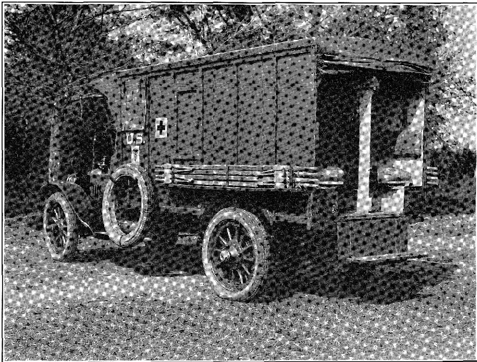
FIG. 21.—Standard G. M. C. ambulance, 1918, with model AA body, rear view
