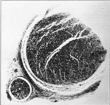
FIG. 229.—Cross section of homo-nerve transplant, stored in liquid petrolatum at 3° C. for 39 days before use, Experiment No. 174, removed 23 days after operation; pyridine-silver preparation. Attention is called to the distinct funicular structure presented by this nerve and the small amount of fibrous tissue development surrounding the nerve
