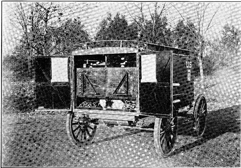
FIG. 30.—Spare parts trailer, rear view
