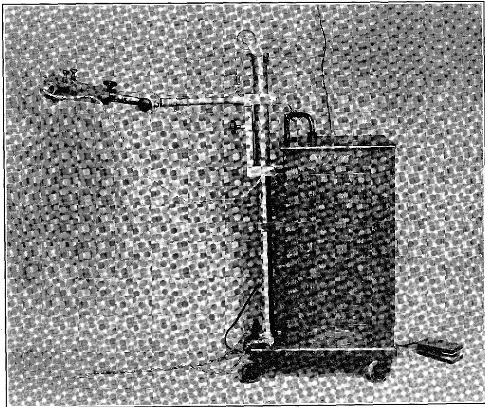
FIG. 38.—Standard bedside X-ray outfit
